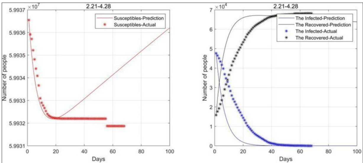
Figure 4. 2020.2.21-2020.4.28 Data fitting result (consider birth rate and natural mortality)
