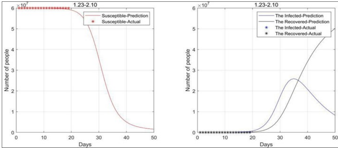
Figure 5. 2020.1.23-2020.2.10 Data fitting result (not consider birth rate and natural mortality)
