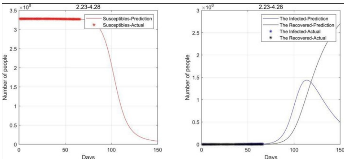
Figure 7. 2020.2.23-2020.4.28 Data fitting result (not consider birth rate and natural mortality)
