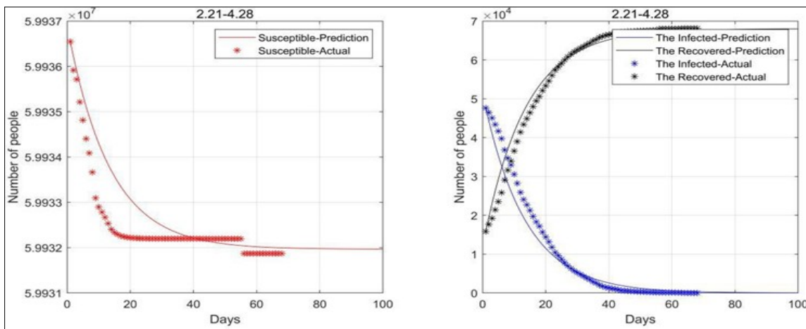
Figure 6. 2020.2.21-2020.4.28 Data fitting result (not consider birth rate and natural mortality)
