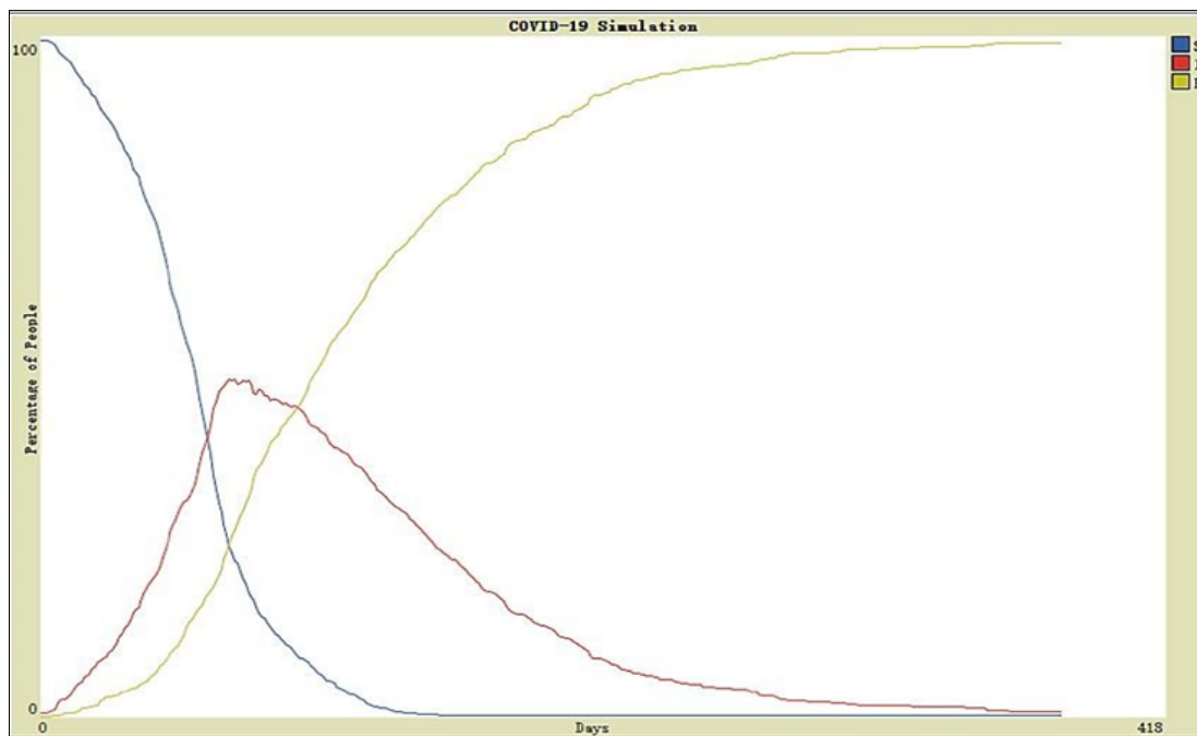
Figure 8. Simulation fitting result from Netlogo
