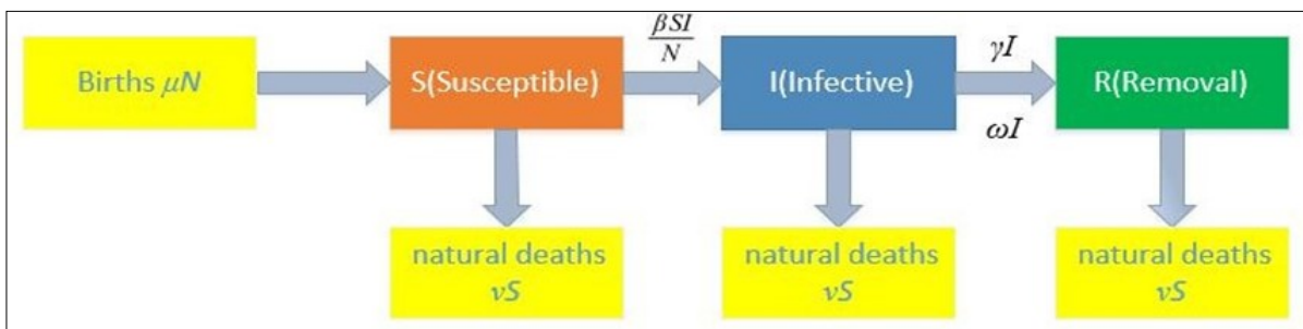
Figure 1. SIR model diagram in Hubei Province (consider births and natural deaths)
